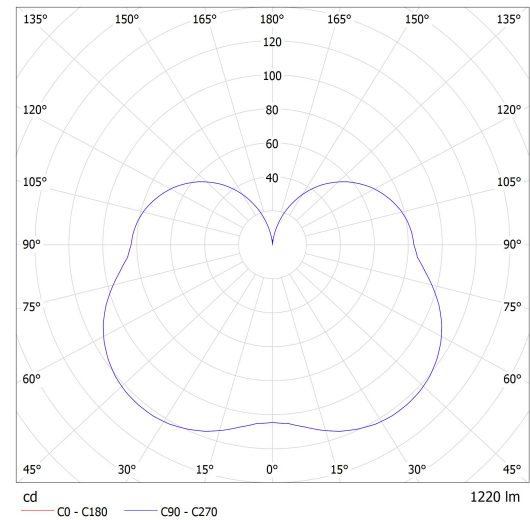
Luminaire: Lucis IC.L1.250.X IZAR C LED Lamps: 1 x LED 2949 G4
