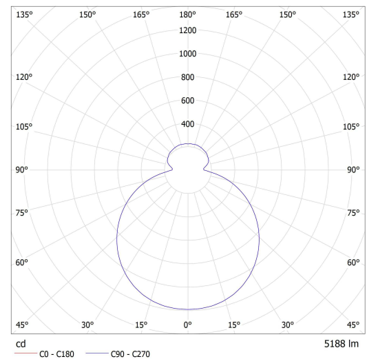
Lucis S46.K1.Z600 ZERO LED / LDC (Polar)
