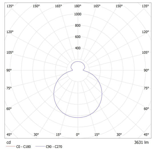
Lucis S34.K2.Z415 ZERO LED / LDC (Polar)
