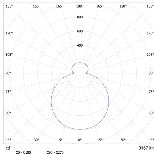
Lucis S34.K1.Z415 ZERO LED / LDC (Polar)
