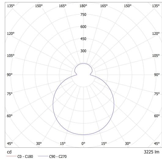
Lucis S43.K4.Z500 ZERO LED / LDC (Polar)
