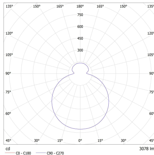
Lucis S43.K3.Z500 ZERO LED / LDC (Polar)
