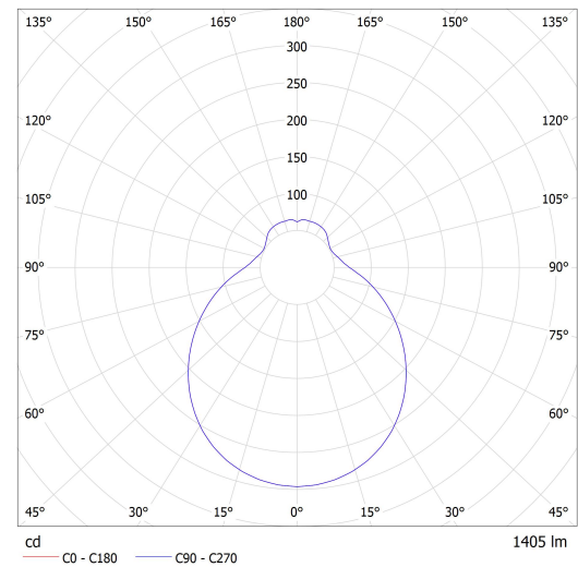
Luminaire: Lucis S24.L1.R4 CAPELLA LED Lamps: 1 x LED G6
