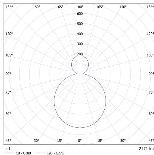
Lucis S34.K2.R450 RONDO LED / LDC (Polar)
