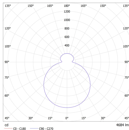
Lucis ZL3.K2.O50 FORUM LED / LDC (Polar)
