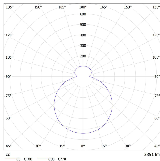
Lucis ZL3.K3.O42 FORUM LED / LDC (Polar)
