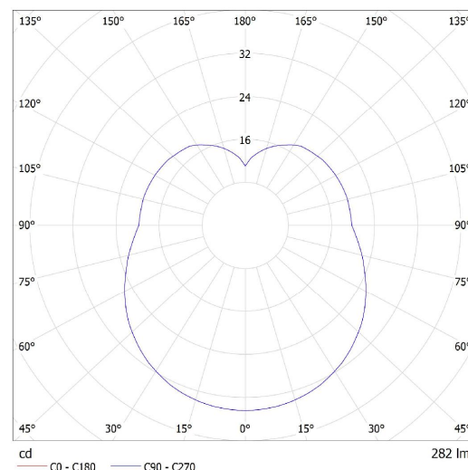
Luminaire: Lucis ZK1.L1.P150 PIA LED Lamps: 1 x LED 4027
