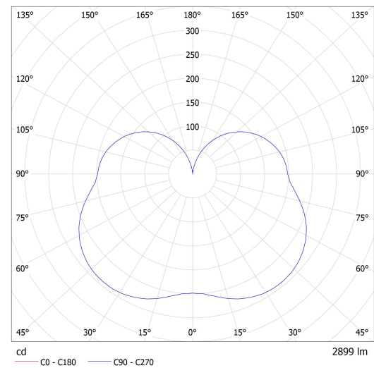
Luminaire IC.K4.440.X IZAR C LED / LDC (Polar)
