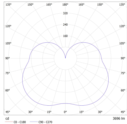
Lucis IC.K1.440.X IZAR C LED / LDC (Polar)
