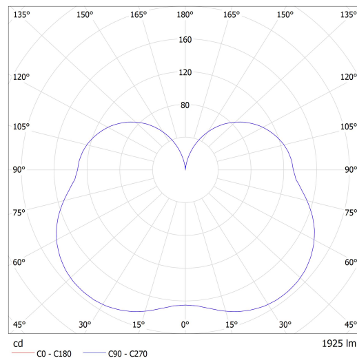
Luminaire IC.K1.250.X IZAR C LED / LDC (Polar)
