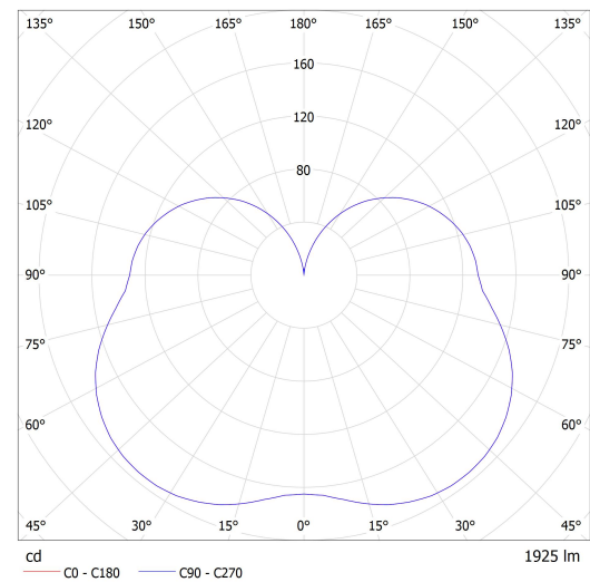
Lucis IC.K1.250.X IZAR C LED / LDC (Polar)
