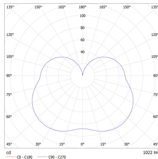
Luminaire IC.K1.150.X IZAR C LED / LDC (Polar)
