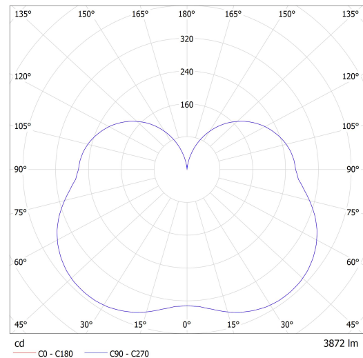
Luminaire: Lucis ZL4.IC.K2.440.X IZAR C LED Lamps: 1 x LED 252/160-G5
