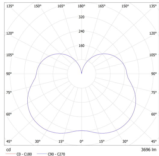
Lucis ZL4.IC.K1.440.X IZAR C LED / LDC (Polar)
