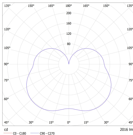
Luminaire: Lucis ZL1.IC.K2.250.X IZAR C LED Lamps: 1 x LED D180-G5
