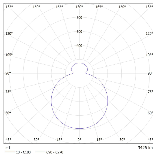
Lucis ZL3.K1.O42 FORUM LED / LDC (Polar)
