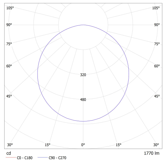
Lucis 28.K2.X_pc(7) Infinity II / LDC (Polar)
