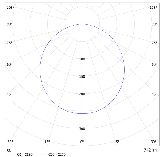
Lucis ZT4.K1.02.X_pc(4) OMNIA LED / LDC (Polar)
