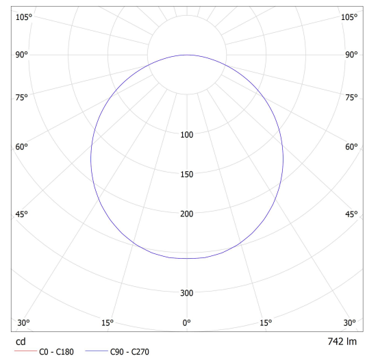
Lucis ZT4.K1.02.X_pc(4) OMNIA LED / LDC (Polar)
