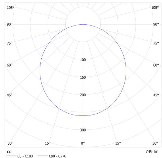
Lucis ZT2.12.K2.O2.X_pc(2) OMNIA LED / LDC (Polar)
