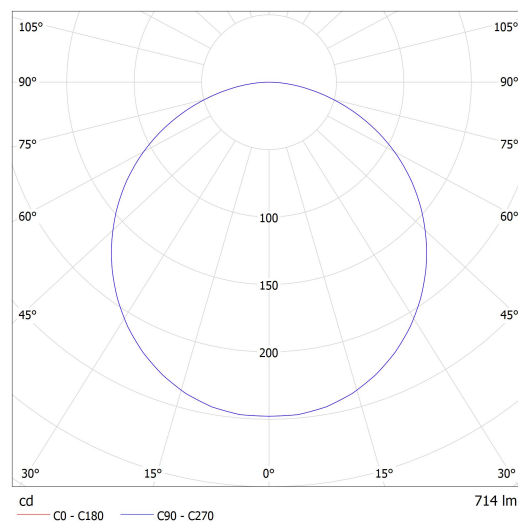
Lucis ZT2.12.K1.02.X_pc(2) OMNIA LED / LDC (Polar)
