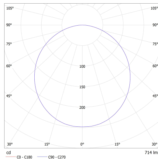
Luminaire: Lucis ZT2.12.K1.02.X_pc(2) OMNIA LED Lamps: 1 x LED G5
