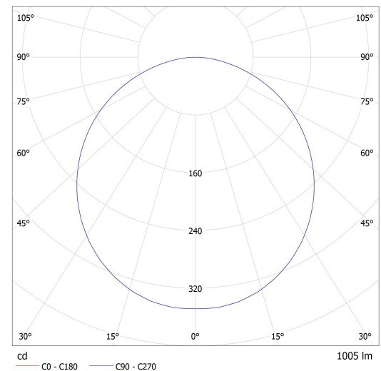
Lucis SR1.K1.O2.X OMNIA LED / LDC (Polar)
