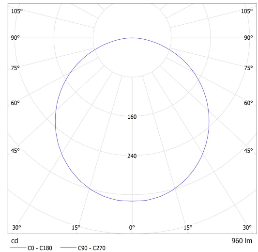
Lucis SR1.K1.02.X OMNIA LED / LDC (Polar)
