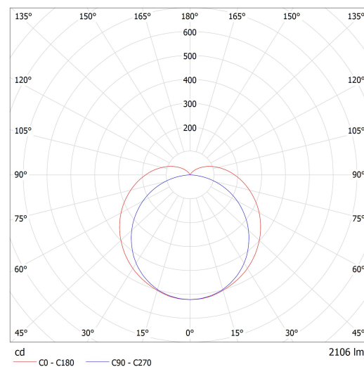
Luminaire: Lucis PS2.L2.X CASTOR LED Lamps: 1 x LED G6
