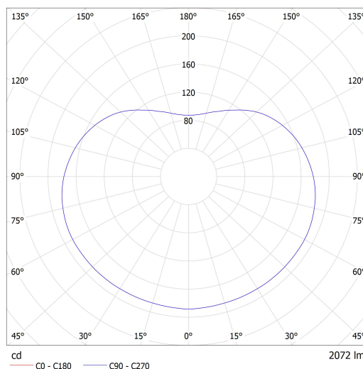
Luminaire: Lucis ZKS.P2.200.X POLARIS ZKS.P LED Lamps: 1 x LED G6
