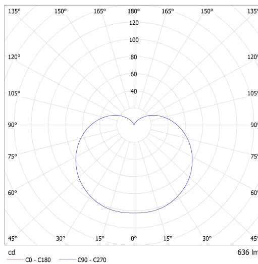
Lucis SR.L1.S200.X SEMILUNA LED / LDC (Polar)
