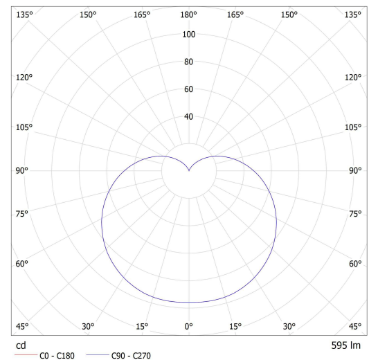
Lucis SR.L1.S200.X SEMILUNA LED / LDC (Polar)
