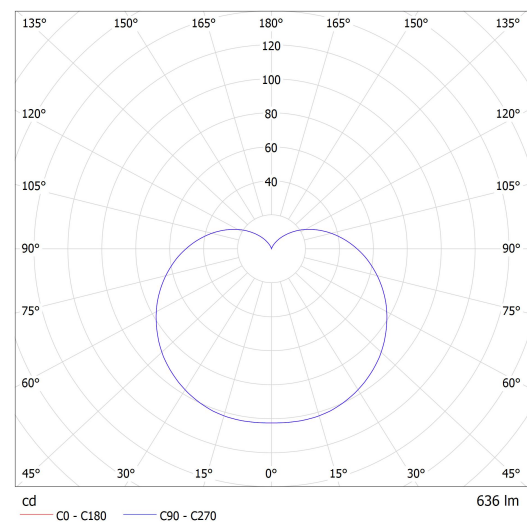
Lucis SR.L1.S200.X SEMILUNA LED / LDC (Polar)
