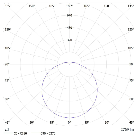
Luminaire: Lucis BS44.K4.P44.X PRIMA LED Lamps: 1 x LED G5
