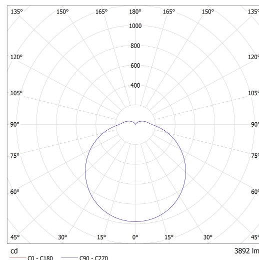
Lucis BS44.K1.P44.X PRIMA LED / LDC (Polar)
