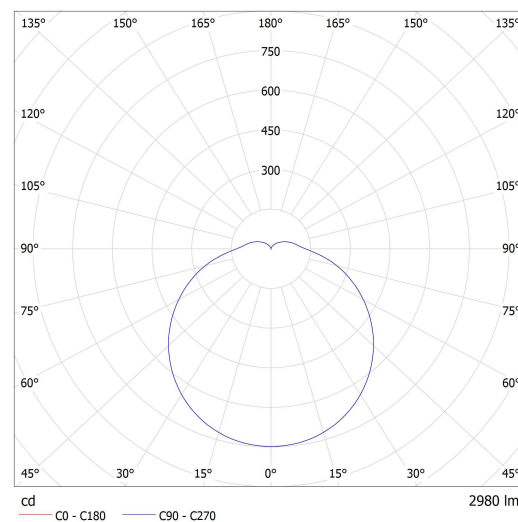
Lucis BS34.K1.P34.X PRIMA LED / LDC (Polar)
