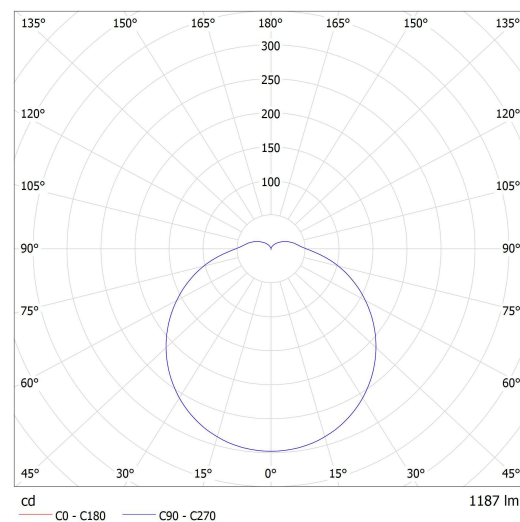
Lucis BS24.K4.P24.X PRIMA LED / LDC (Polar)
