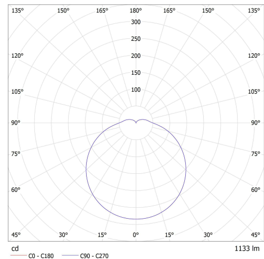
Lucis BS24.K3.P24.X PRIMA LED / LDC (Polar)
