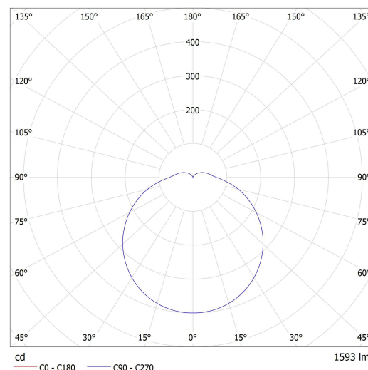
Lucis BS24.K1.P24.X PRIMA LED / LDC (Polar)
