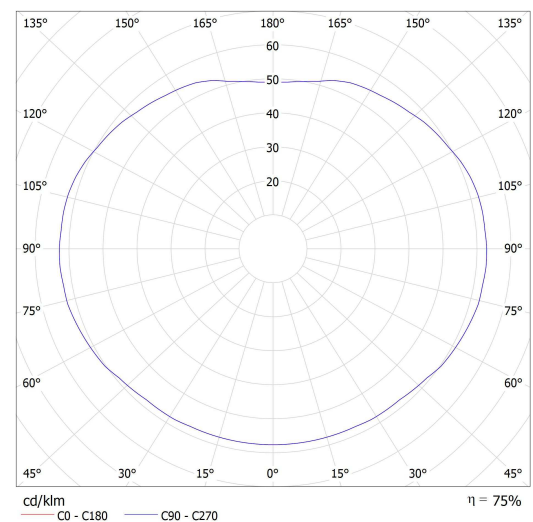
Lucis ZK2.11.GC.61R GEO / LDC (Polar)
