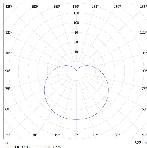
Luminaire: Lucis ZL.L2.C.X CAPSULE LED Lamps: 1 x LED G5
