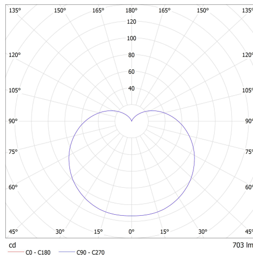
Luminaire: Lucis ZL.L2.C20.X CAPSULE LED Lamps: 1 x LED G6
