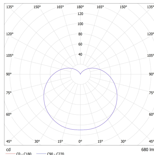
Luminaire: Lucis ZL.L1.C.X CAPSULE LED Lamps: 1 x LED 0481212-3 F1
