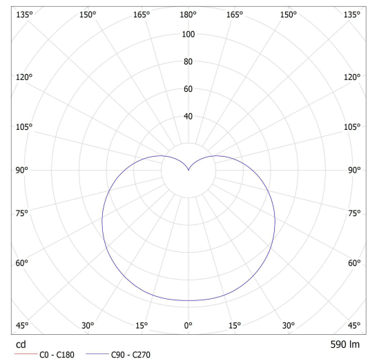
Lucis ZL.L1.C.X CAPSULE LED / LDC (Polar)
