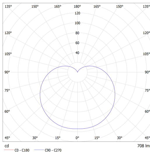
Lucis ZT.L2.S200.X SEMILUNA LED / LDC (Polar)
