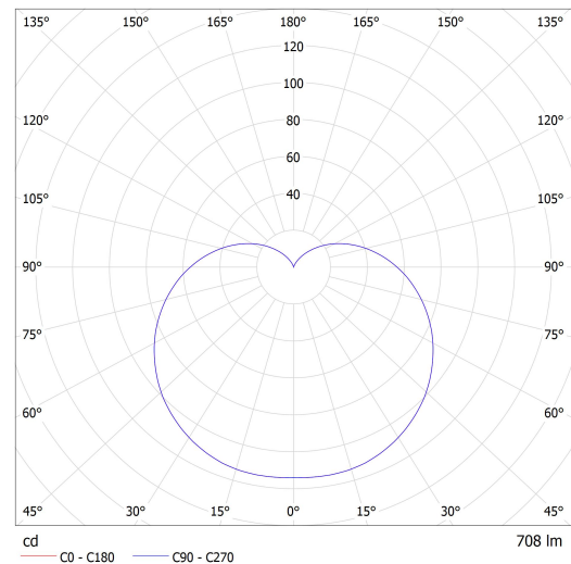
Luminaire: Lucis ZT.L2.S200.X SEMILUNA LED Lamps: 1 x LED G6
