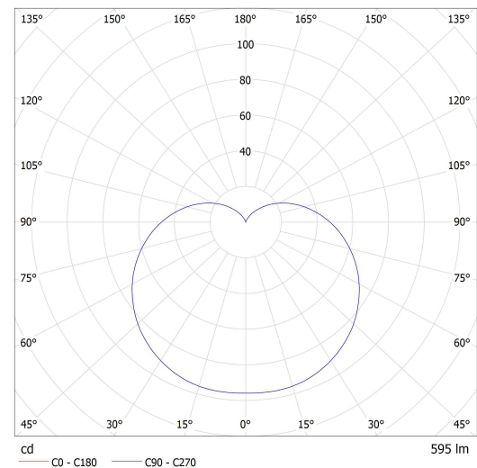
Lucis ZT.L1.S200.X SEMILUNA LED / LDC (Polar)
