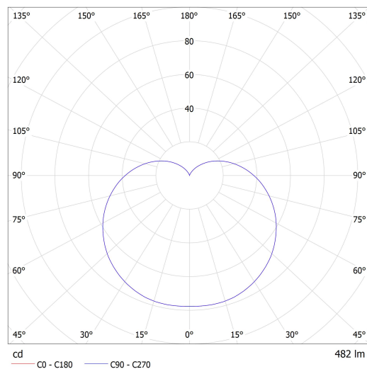
Luminaire: Lucis ZT.L1.S115.X SEMILUNA LED Lamps: 1 x LED G6
