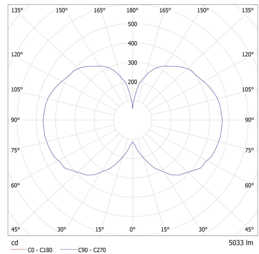
Lucis ZK.L2B.M620 PA MAIA LED / LDC (Polar)
