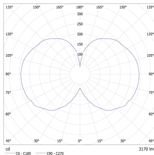
Lucis ZK.L3B.M500 PA MAIA LED / LDC (Polar)
